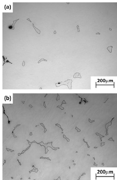
Fig. 6. Microstructure of (a) 10Mg SF, (b) 10Mg MF.
