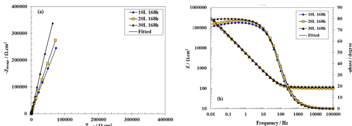
Fig. 3. (a) Nyquist and (b) Bode plot of 10L, 20L, and 30L on AISI 304 substrate.
