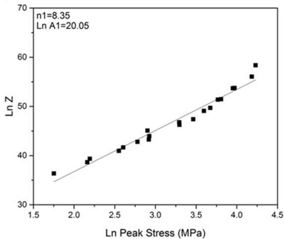
Fig. 7. The relationship between Ln Z vs. Ln peak stress.
