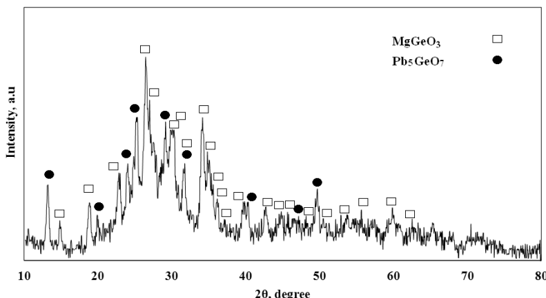
Fig. 4. The XRD pattern of as-quenched 65\text{GeO}_2\text{-}15\text{PbO}\text{-}10\text{MgO}\text{-}10\text{MgF}_2 sample after annealing at 800^\circ\text{C} for 60 minutes.
