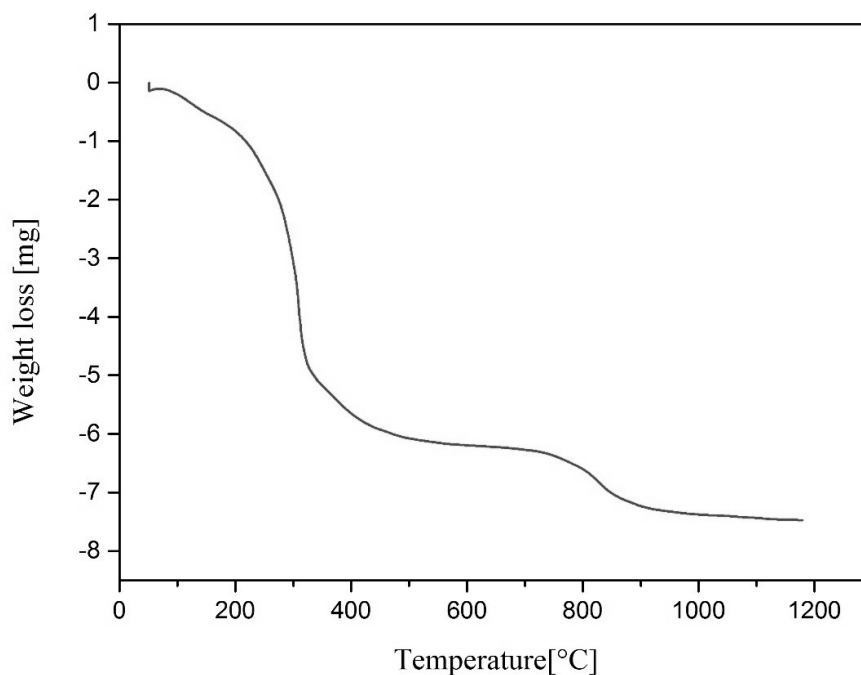
Fig. 3. The TG curve of dried sample with the rate of 10^\circ\text{C}/\text{min} in air.
