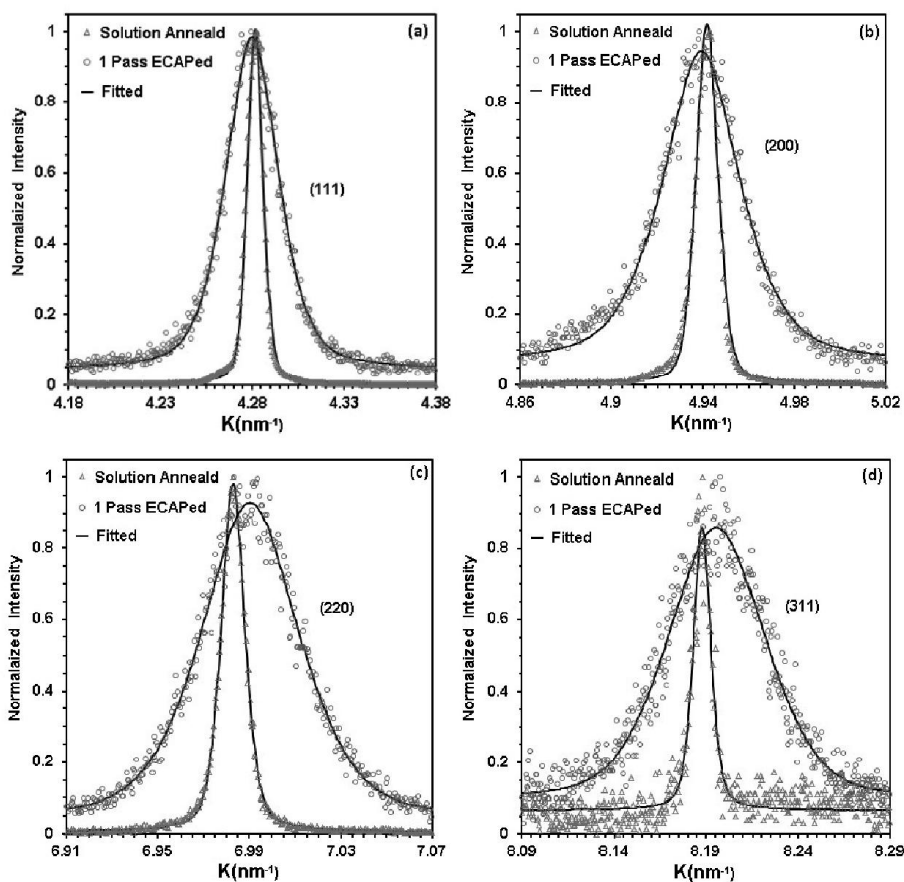
Fig. 2. Measured and fitted XRD peaks after normalizing vs. diffraction vector on the solution annealed and the deformed sample (a) (111) diffraction; (b) (200) diffraction; (3) (220) diffraction; (d) (311) diffraction
