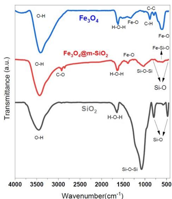
Fig. 2. FTIR spectra of \text{SiO}_2 , \text{Fe}_3\text{O}_4 , \text{Fe}_3\text{O}_4@m\text{-SiO}_2 NPs
