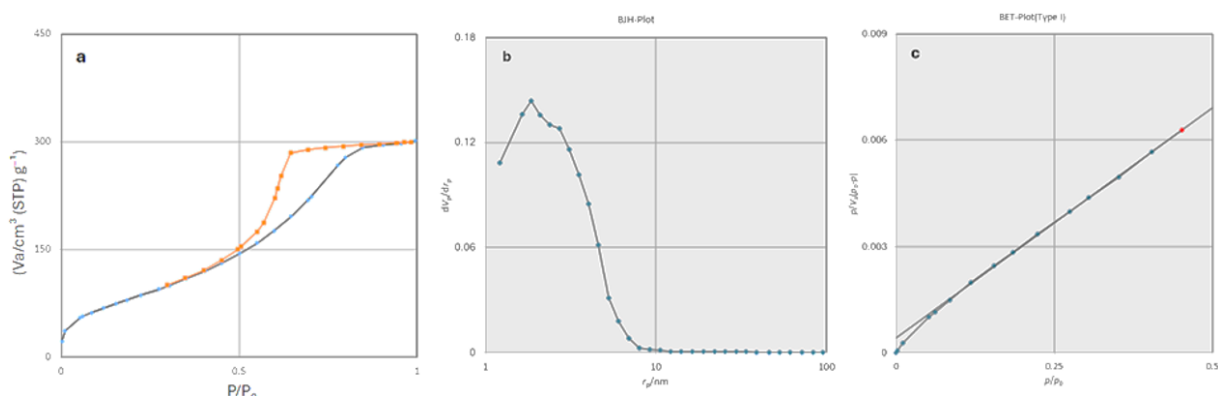
Fig. 7. a) Nitrogen Adsorption-Desorption Isotherm of \text{Fe}_3\text{O}_4@m\text{-SiO}_2 NPs, b) The pore size distribution plot of the \text{Fe}_3\text{O}_4 m-SiO 2 NPs, and c) The BET plot of the \text{Fe}_3\text{O}_4@m\text{-SiO}_2 NPs
