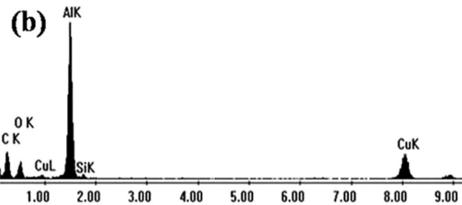
Fig. 8. (a) BFI of Al-5%SiC nanocomposite powder obtained after 25 h of ball-milling and (b) EDS analysis of the region marked in (a).
