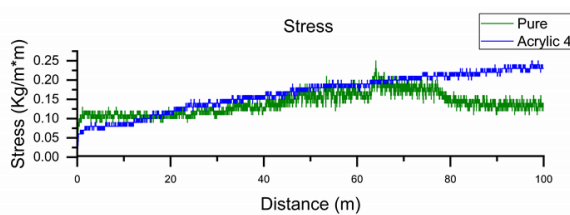
Fig. 8. Comparison of wear stress of pure Acrylic and Acrylic 4
