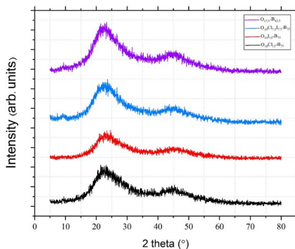
Fig. 3. XRD pattern of the prepared glass sample
