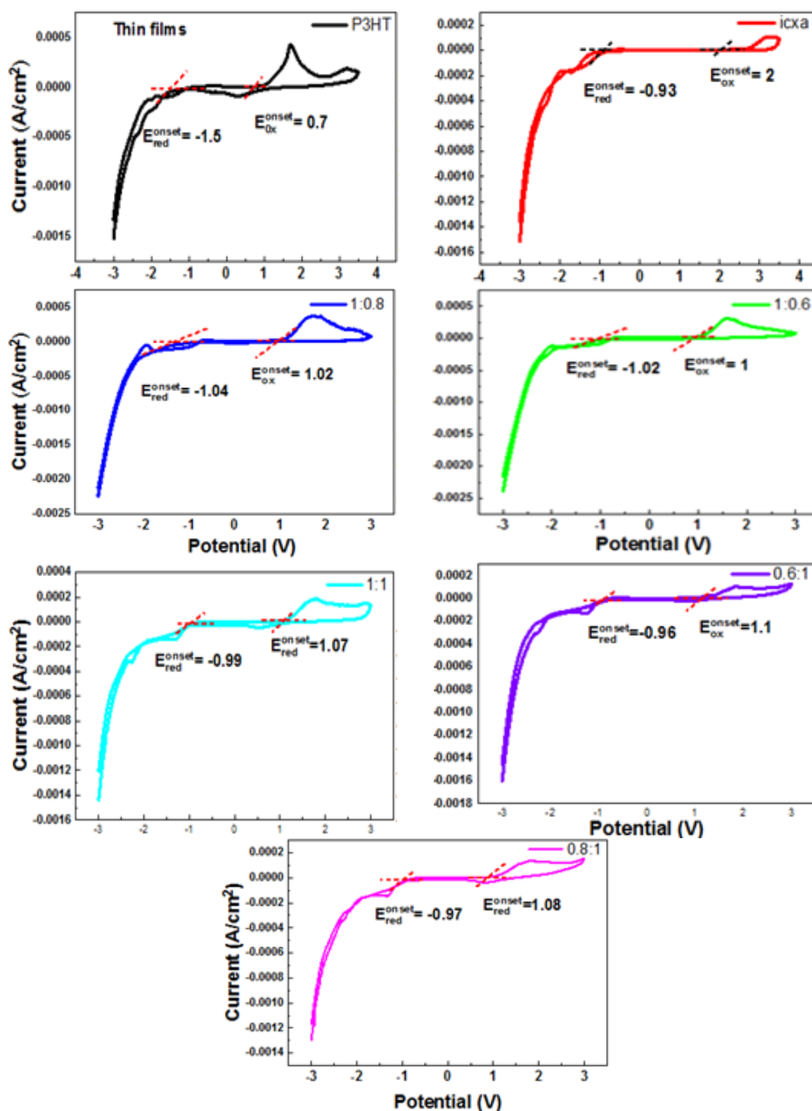
Fig. 8. Cyclic voltammety curves for P3HT:ICxA blends. Cross-dashed lines were used to estimate position of E_{\text{red}} and E_{\text{ox}} .
