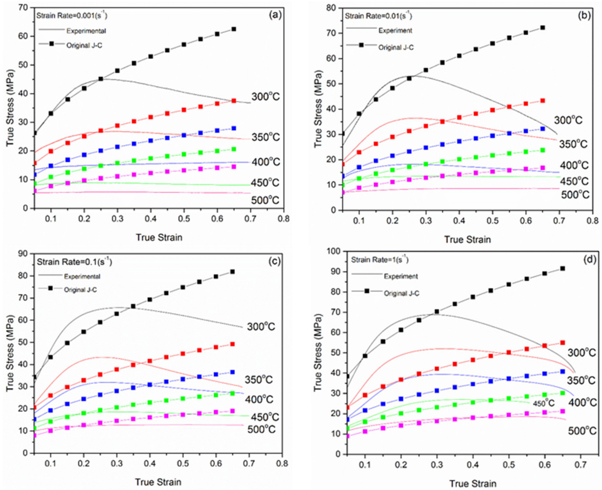
Fig. 6. Comparison between experiment and predicted flow stress by J-C model at different temperatures and strain rates of (a) 0.001 s -1 , (b) 0.01 s -1 , (c) 0.1 s -1 and (d) 1 s -1 .
