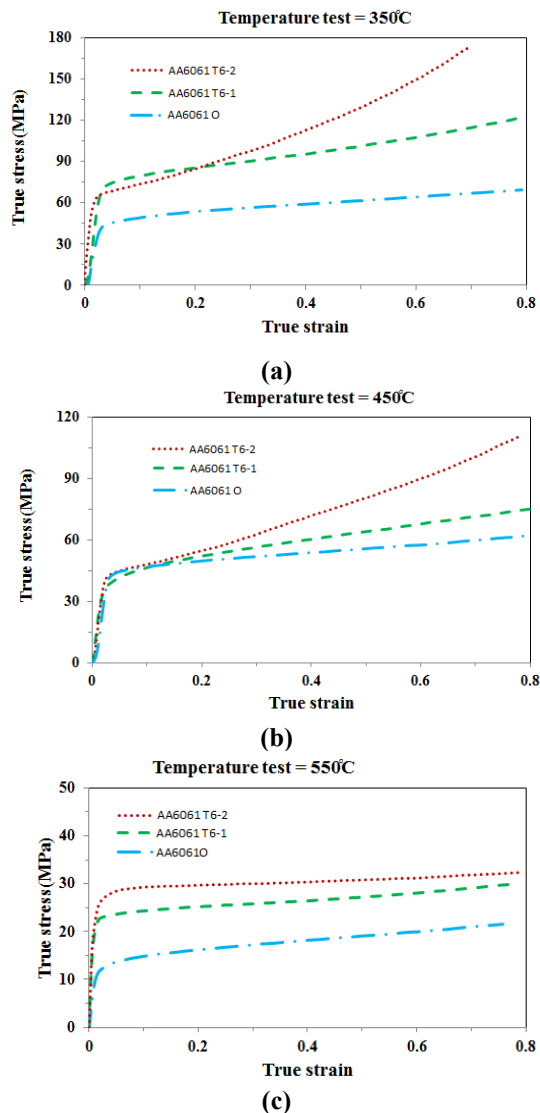
Fig. 9. True stress-true strain curve of AA6061 O, AA6061 T6-1, and AA6061 T6-2 during hot compression deformation at \dot{\epsilon} = 0.1 \text{ s}^{-1} and different temperatures of (a) 350, (b) 450, and (c) 550°C.
