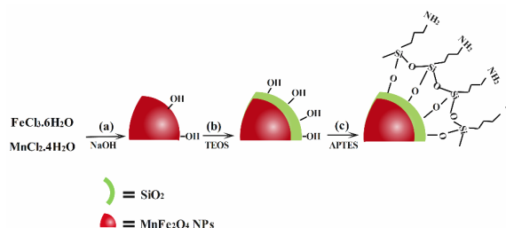
Fig. 2. Schematic illustration of MnFe 2 O 4 @SiO 2 -NH 2 nanocomposite particles preparation: (a) synthesis of MnFe 2 O 4 NPs, (b) formation of SiO 2 shell, and (c) synthesis of MnFe 2 O 4 @SiO 2 -NH 2 NPs
