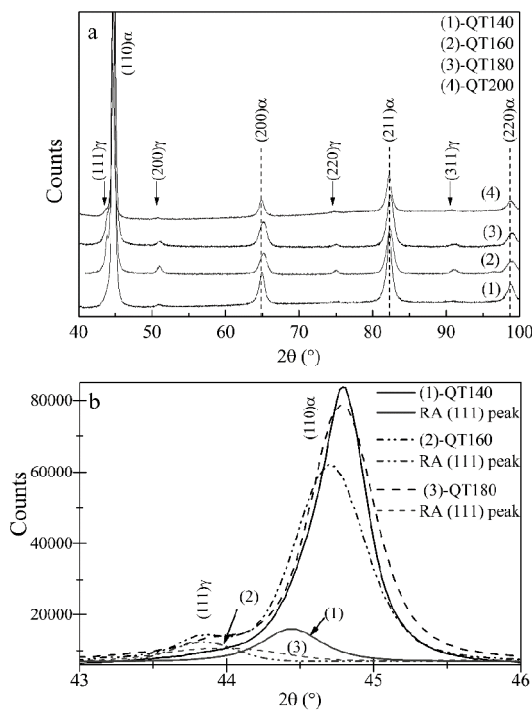
Fig. 2. (a) X-ray diffraction pattern of Q&P samples quenched to different QT. (b) Deconvolution lines of (111)γ and (110)α main peaks.
