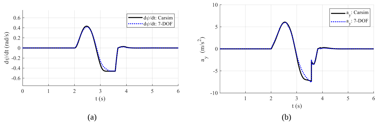
Figure 6: Validation of the 7-DOF model in MATLAB/Simulink with Carsim. (a) Yaw rate (b) Lateral acceleration.
